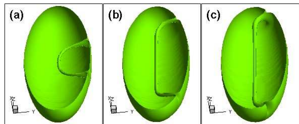
FIG. 2: Single U vortex configurations for \Omega/\omega_x = 0.42 (a), 0.58 (b), 0.78 (c).
